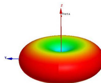
Directional pattern of the antenna
